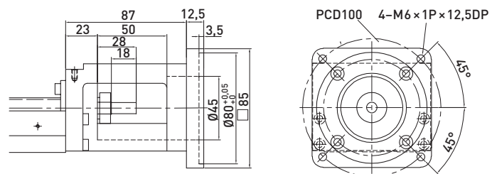
F7 motor-adapterkarima
