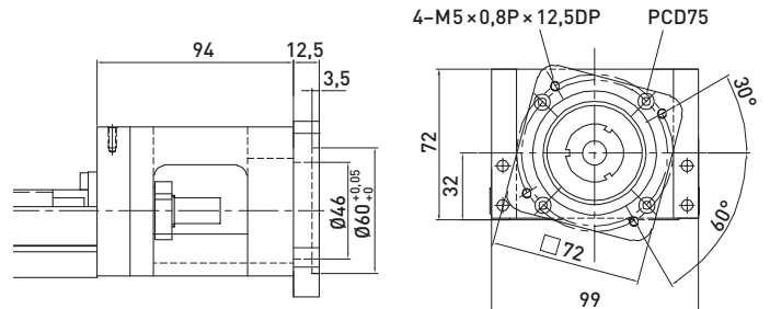
F7 motor-adapterkarima
