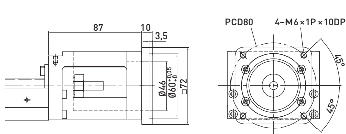
F9 motor-adapterkarima
