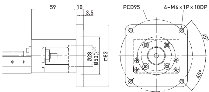
F9 motor-adapterkarima
