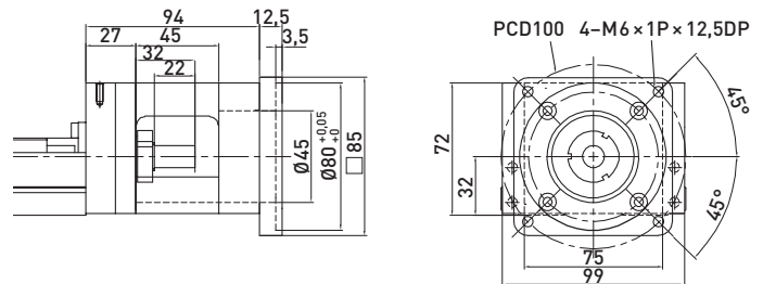
F5 motor-adapterkarima
