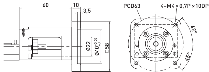
F5 motor-adapterkarima
