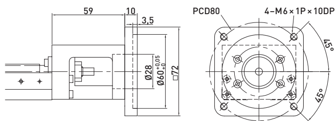
F7 motor-adapterkarima
